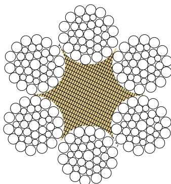
6X36WS+FC
