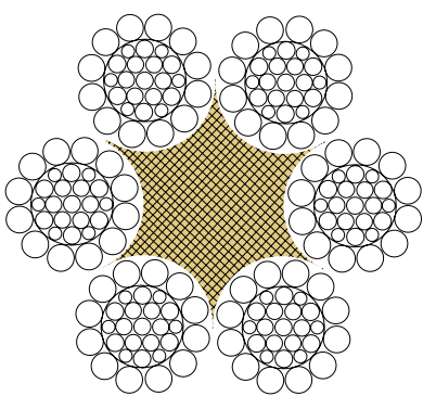
6X31WS+FC
